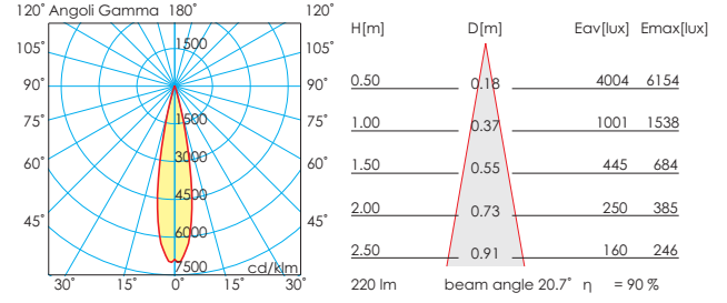
20° @700mA
